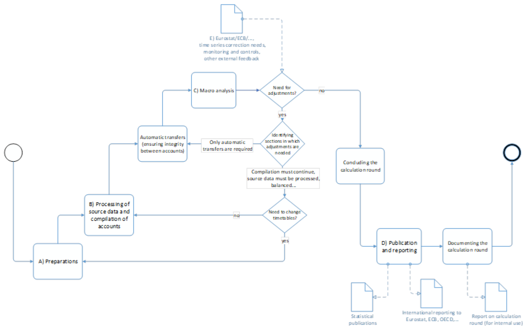
Figure 1-3: Compilation round
