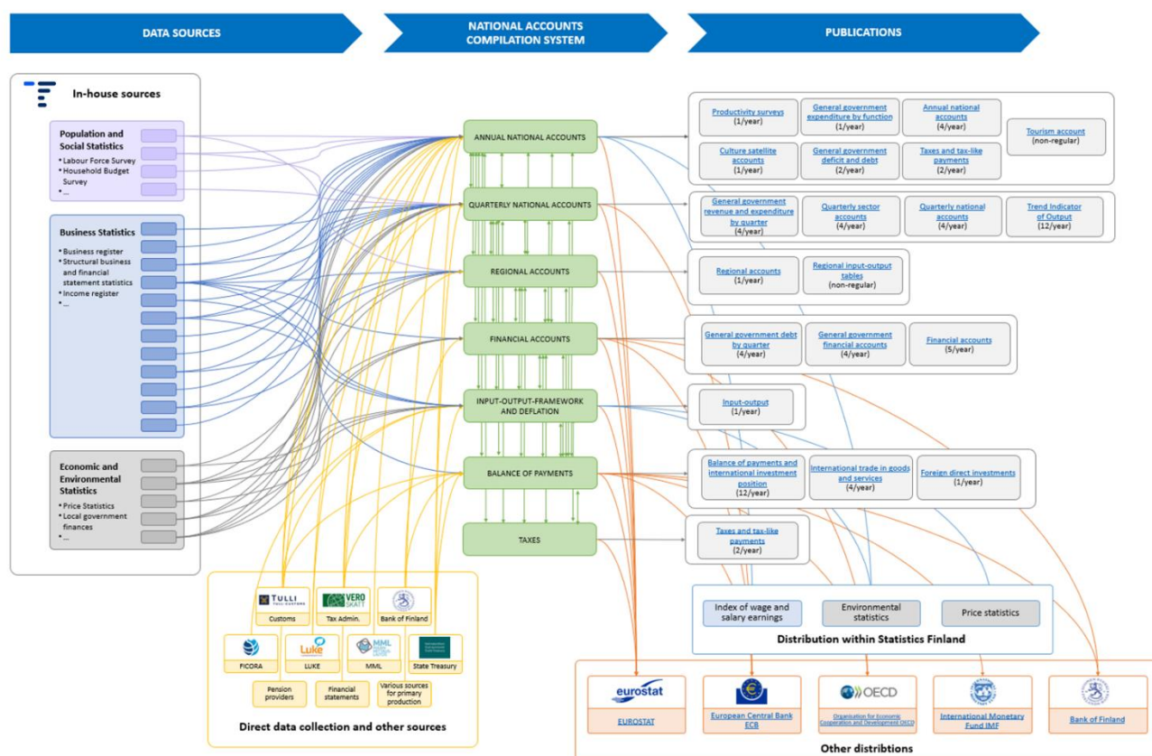
Figure 1-7: Data flow
